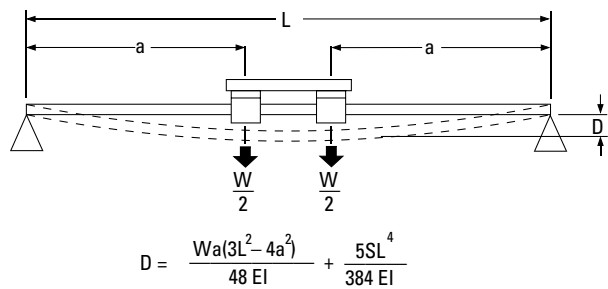
Simply Supported 60 Case LinearRace with Two Blocks
