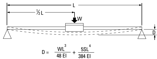
Simply Supported 60 Case LinearRace with One Block
