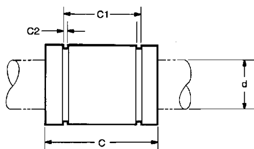
MultiTrac Ball Bushing Linear Bearings (Closed Type) (Dimensions in mm)
