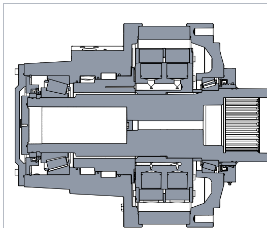
Figure 25. 1-speed motor.
