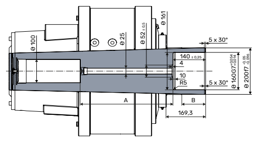
Figure 19. Dimensions of the shaft type 5A, shrink disc.
