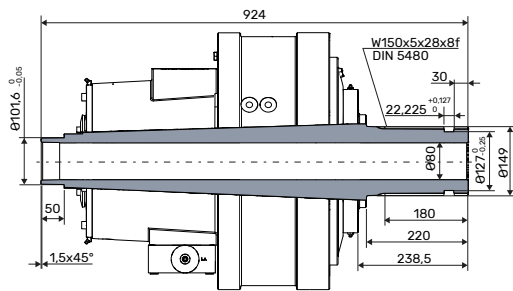
Figure 16. Dimensions of the shaft type 3A, through splines W150.
