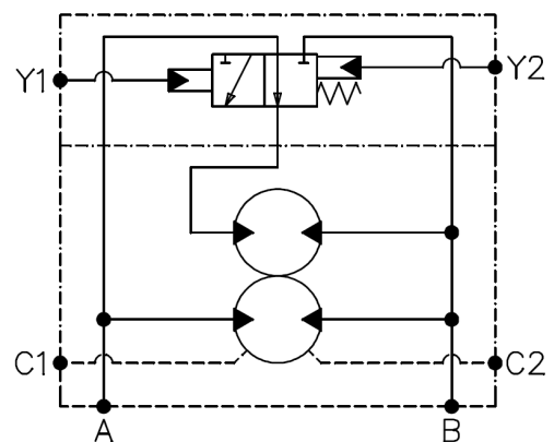
Figure 28. Hydraulic circuit, 2-speed motor.
