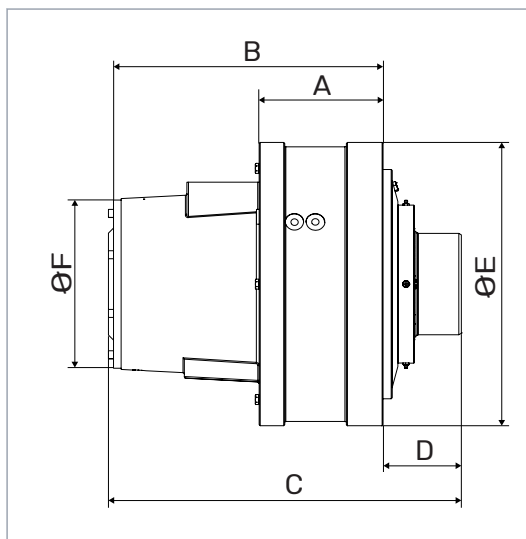
Figure 5. Shaft types 1A, 1B, 1C, 1D, 4A, 4B and 5A.
