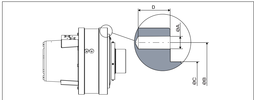
Figure 21. Dimensions of the housing interface.
