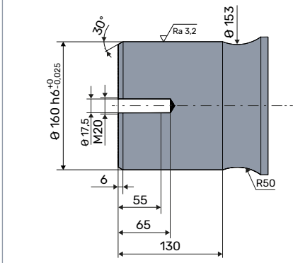
Figure 20. Dimensions of the recommended customer shaft design for type 5A. Material ex. 42CrMo4.
