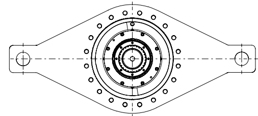
Figure 23. Double ended torque arm.
