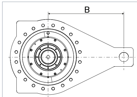
Figure 22. Torque arm length.
