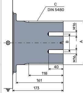
Figure 17. Dimensions of the shaft types 4A and 4B. Solid shaft W150 / W180.
