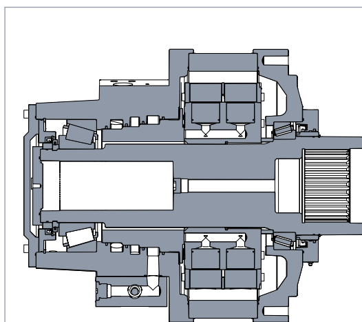
Figure 27. 2-speed motor.
