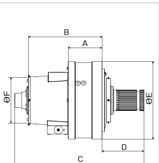
Figure 6. Shaft types 2A, 3A and 3B.
