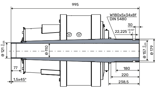
Figure 18. Dimensions of the shaft type 3B, through splines W180.
